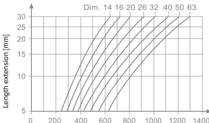
Bending leg length for TECElogo pipes
