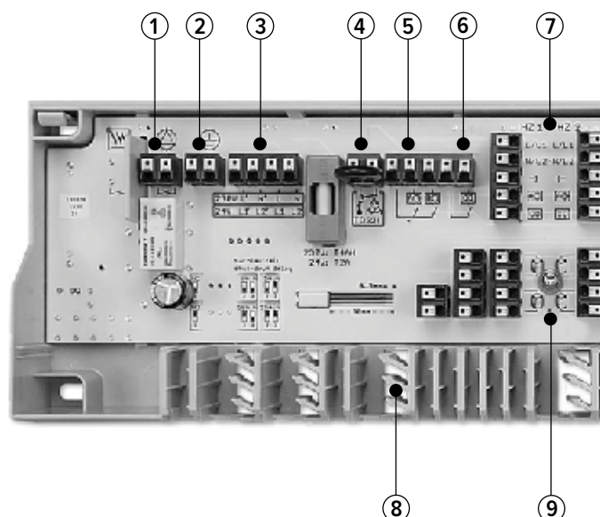
TECEfloor connection unit (Standard Plus)
