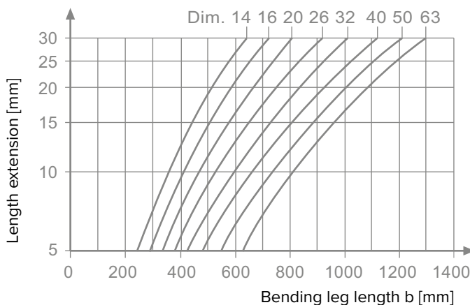
Bending leg length for TECEflex pipes
